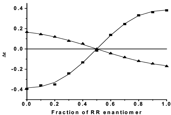
Fig. 7 Variation of the molar ellipticity as a function of the SS/RR ratio for the nickel(II) (▲) and copper(II) (■) complexes.
